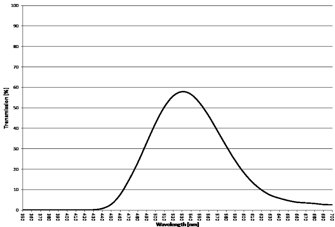
Spectral Transmittance
