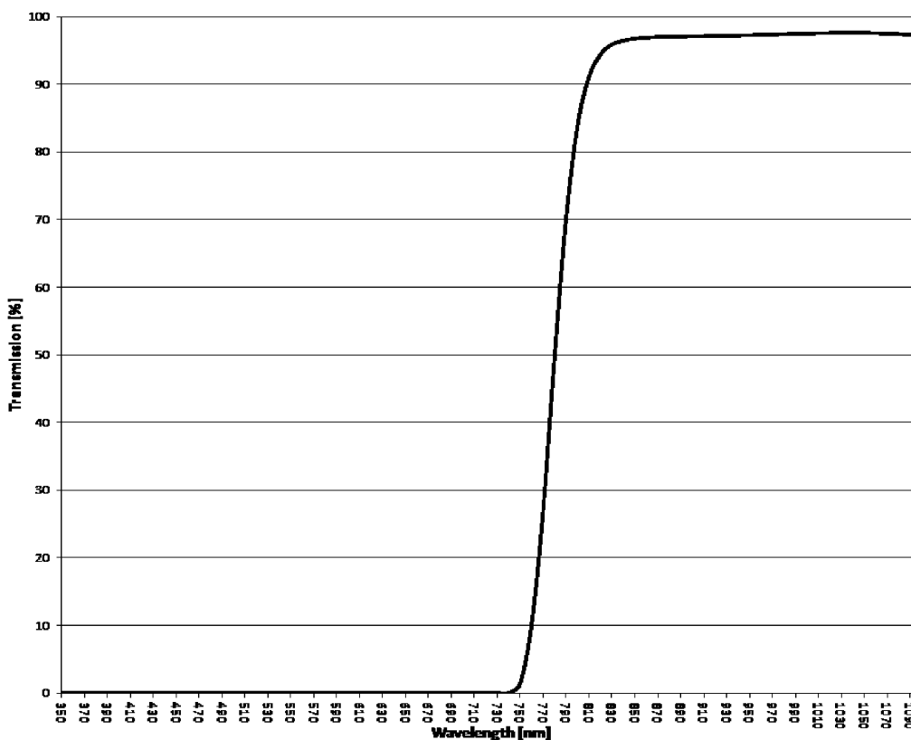
Spectral Transmittance
